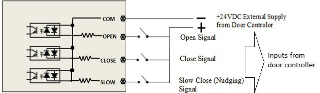
Figure 3 Connections with External Supply
